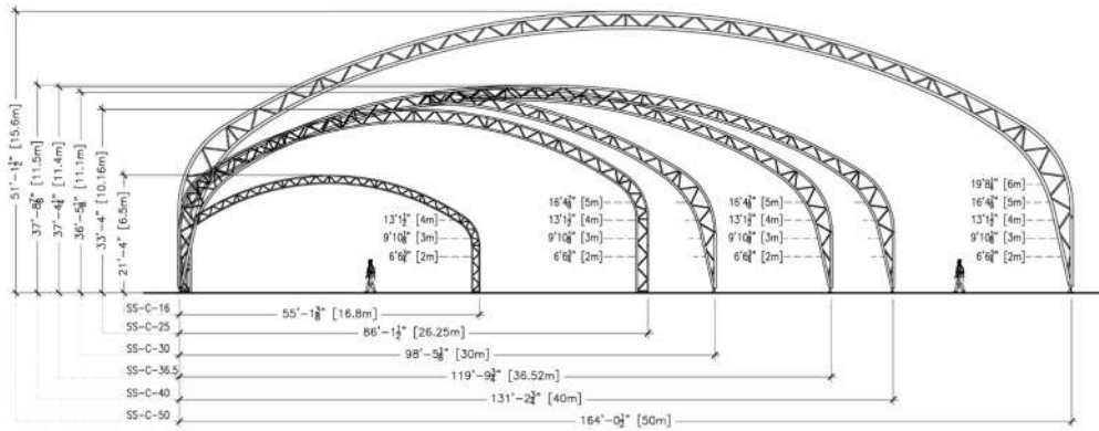
SUPA-SPAN-C-16-25-30-36.5-40-50-CURVED PROFILE SUPA-SPAN STRUCTURE IS MODULAR ON 3M BAYS SUPA-SPAN STRUCTURES 30M, 36M, 40M AND 50M ARE MODULAR ON 6M BAYS
